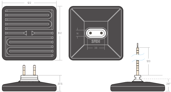
SFEH SQUARE FLAT ELEMENT HOLLOW Tolerances apply, all dimensions mm. * Face of reflector - face of element using 0.75 mm reflector, mounting hole size 6 x 42 mm. Element supplied with Wave Spring and Clip CE 23906
