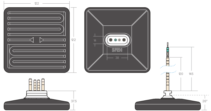
SFEH + TC SQUARE FLAT ELEMENT HOLLOW WITH TYPE K THERMOCOUPLE Tolerances apply, all dimensions mm. * Face of reflector - face of element using 0.75 mm reflector, mounting hole size 6 x 42 mm. Element supplied with Wave Spring and Clip CE 23906
